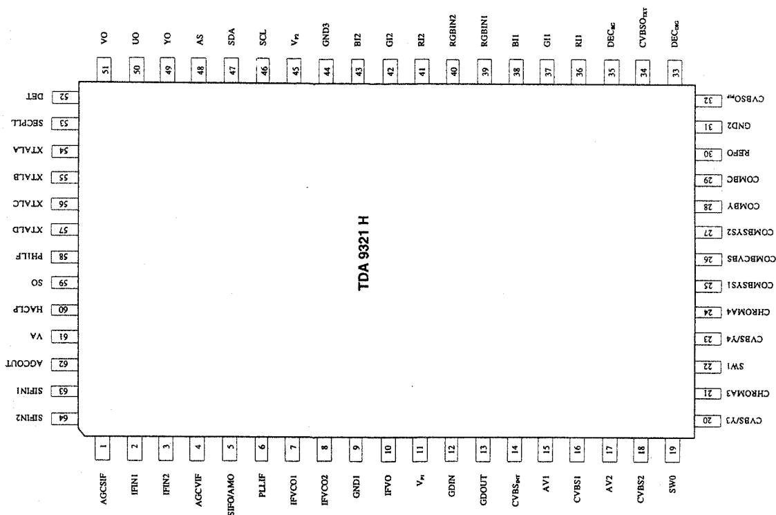
Rinning diagram of QFP-64
