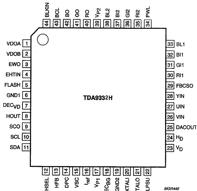
Pinning diagram of QFP44
